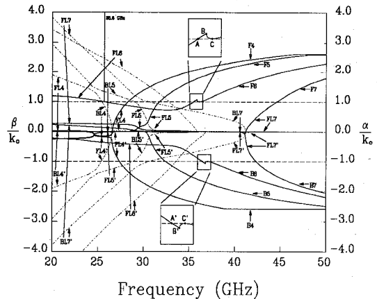
Fig. 4. The dispersion characteristics of the Type II structure defined in Fig. 1. Only four sets of higher-order modes numbered from 4-7 are presented. The solid lines represent the normalized propagation constants \beta/k_0 and correspond to the vertical axis on the left-hand side. The dash-dot lines represent the normalized attenuation constants \alpha/k_0 and correspond to the vertical axis on the right-hand side. The most visible spectral gaps of the sixth mode pair are enlarged in the insets. Critical points A, B , and C ( A', B' , and C' ) are also plotted in the insets and defined in the text.
