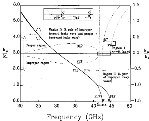
Fig. 3. The frequency-dependent variation of the transverse wavenumber k_{yo} of the seventh mode pair of the Type I structure. The dash-dot lines represent the normalized imaginary parts k_{yi}/k_0 and correspond to the vertical axis on the right-hand side. The solid lines represent the normalized real parts k_{yr}/k_0 and correspond to the vertical axis on the left-hand side. The real parts are always greater than or equal to zero. Therefore, the behavior of each wave type is characterized by the imaginary part. When k_{yi} > 0 , the wave is proper, and when k_{yi} < 0 , the wave is improper.
